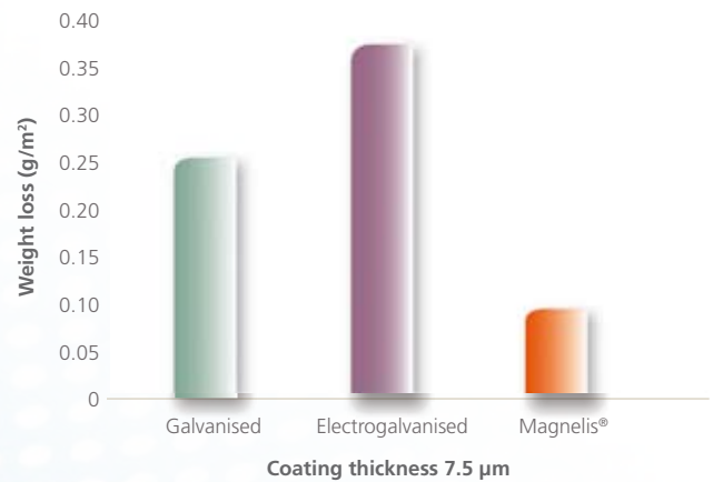
Lubrication: Fuchs 4107S in excess Powdering behaviour comparison between metallic substrates expressed in weight loss (g/m²)
