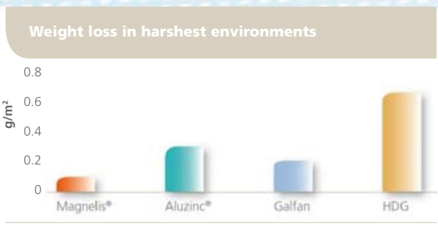
Measurement of mass loss pH: 11.7 - Solution with 5% NH 3 - T: 20°C - Test duration 24 h
