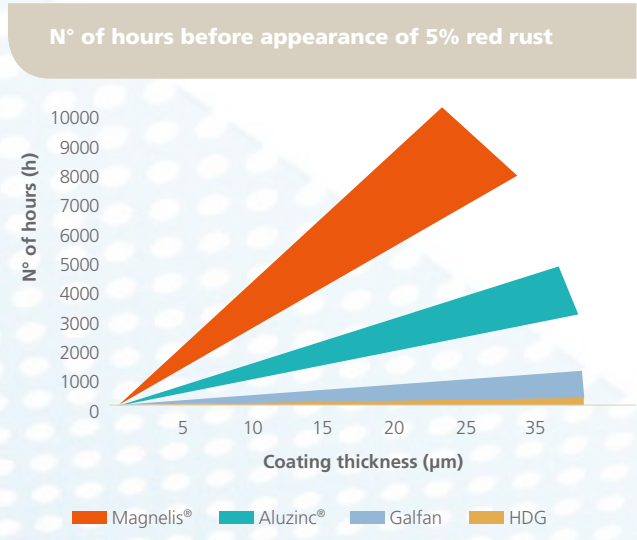
Corrosion resistance by salt spray test (average): Magnelis®: > 200 h/µm - Aluzinc®: ±100 h/µm - Galfan: ± 25 h/µm Hot dip galvanised (HDG): ± 8-10 h/µm
